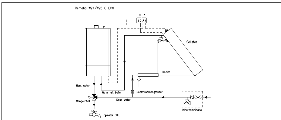
Afb 18. Principeschema Remeha W21/28c ECO met Remeha Solistor zonneboiler 00C00HS00001
